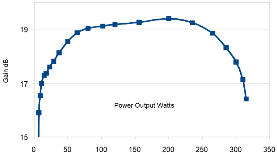
Power Output vs Gain
