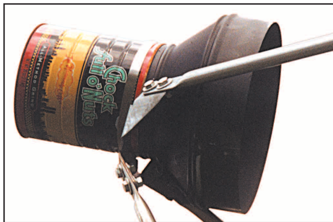
Since we intend to use the VSA at L-band, on a frequency of 1296 MHz, one can scale the dimensions of the standard C-band feed by a factor of three. As is the amateur tradition this feedhorn is constructed from low-cost materials!
