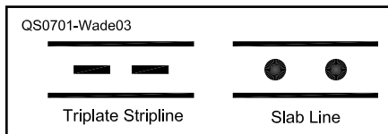
Figure 3 — Common cross-section geometries for directional couplers.
