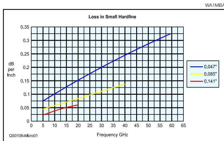
Figure 1—Loss in small semi-rigid coaxial line.
