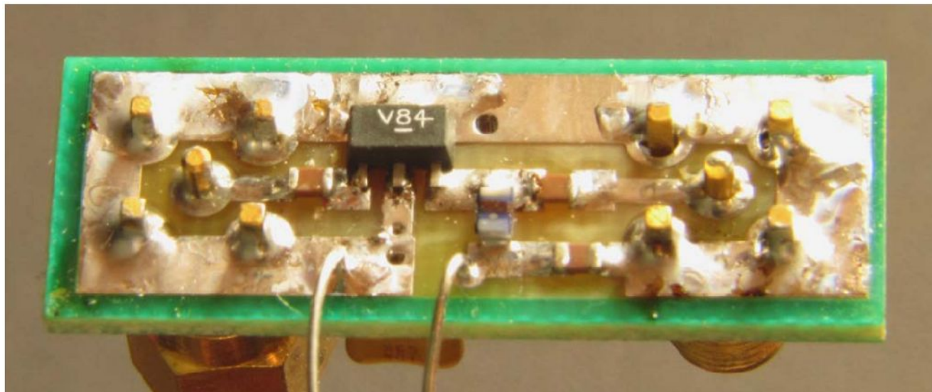
Figure 1- GVA-84 Microwave Amplifier
